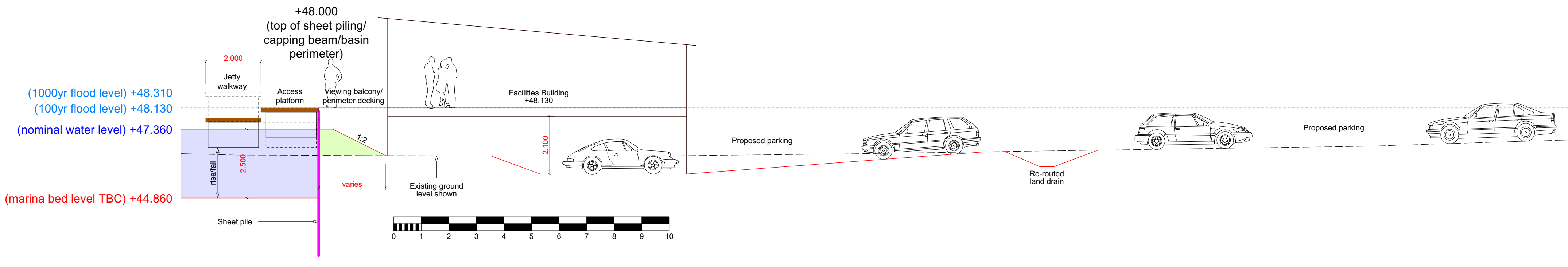
Typical Section Thru Proposed New Basin, Bund & Building Scale 1:100
