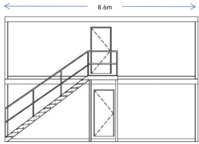
Eastern Elevation
