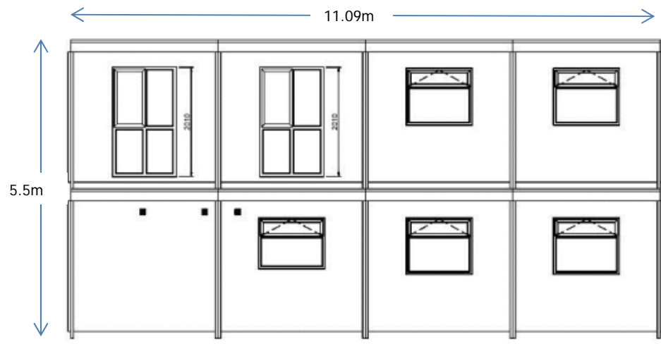
Northern Elevation
