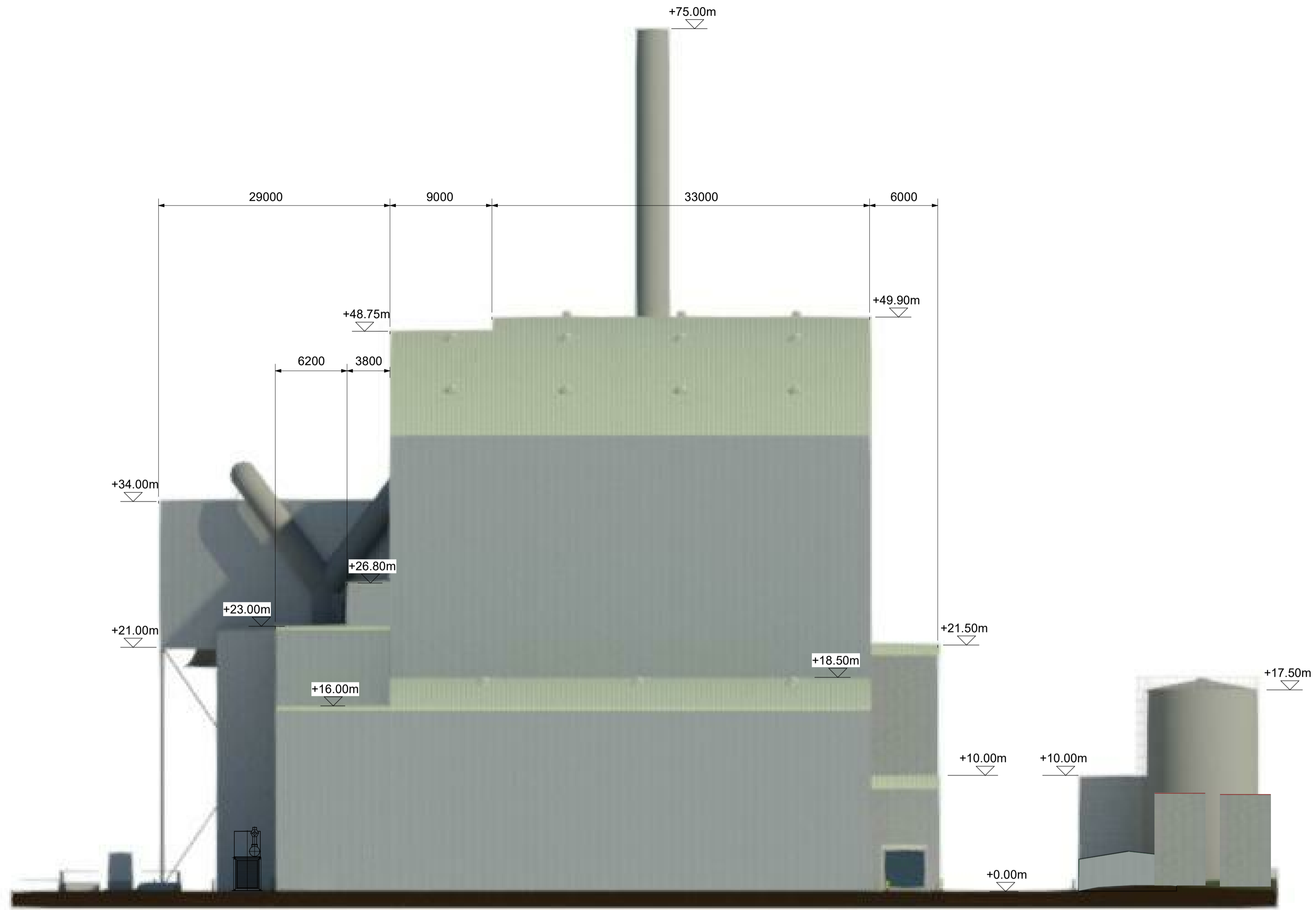
C East Elevation 1:1 NTS
