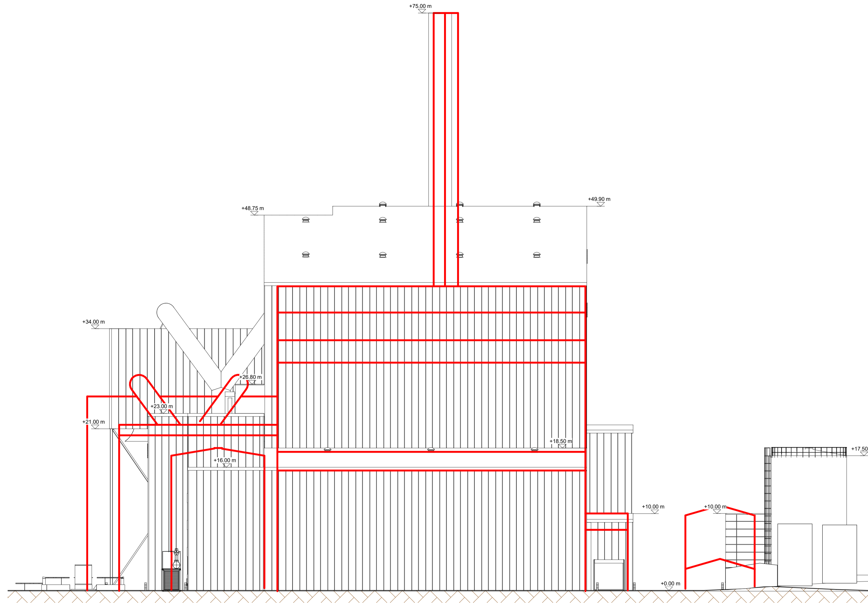
2 East Elevation 1 : 250
