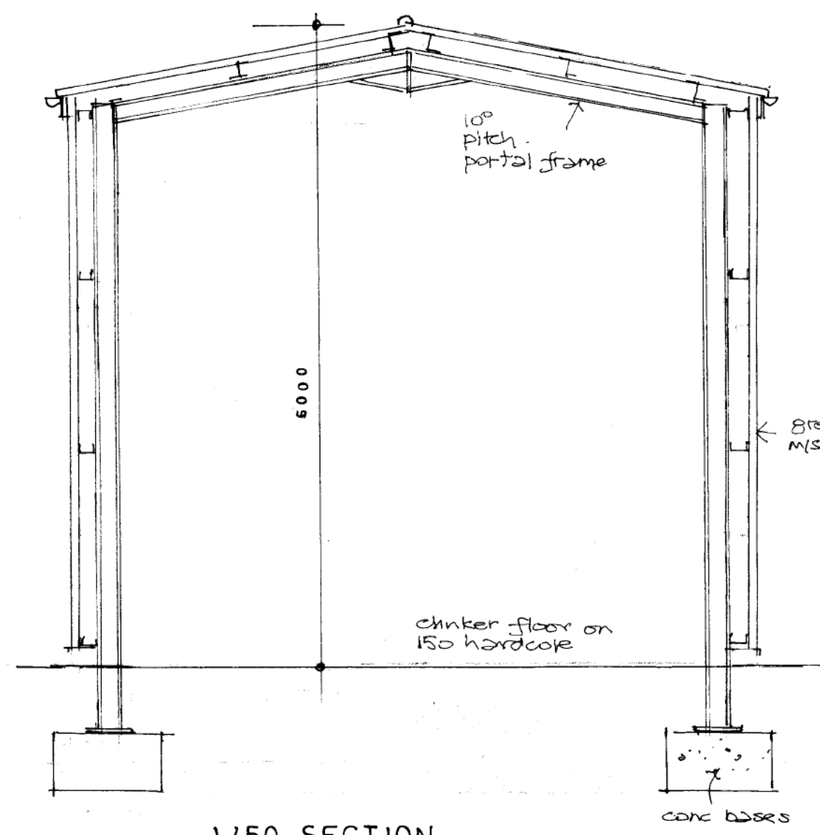
1/50 SECTION
